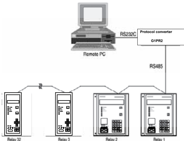
Figure 4 - Relay Setting and Monitoring System
